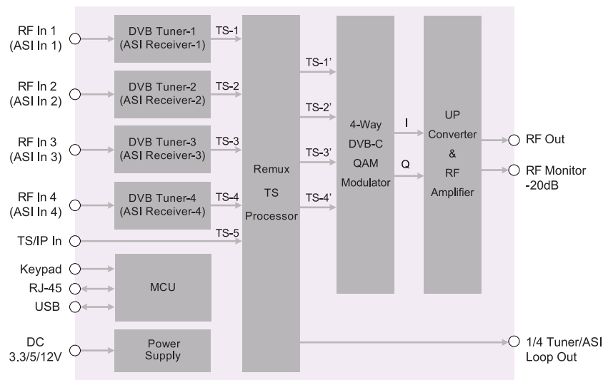
DMM-2400TM Functional Block Diagram
